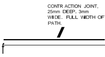
TRANSVERSE CONTRACTION JOINT AT 3000 MAX. SPACING
