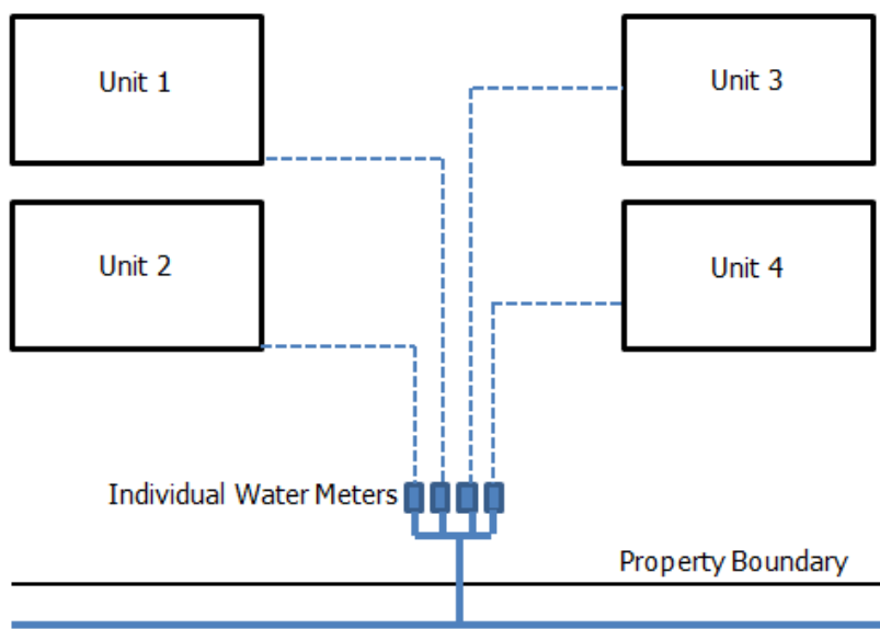
Figure 1: Strata and Community Title water connections utilising a master meter and sub meter arrangement.
